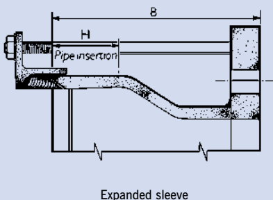
Expanded sleeve
